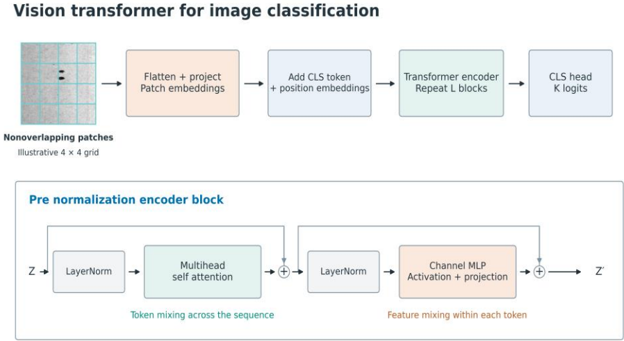
Figure 2. Patch embedding and a conventional pre-normalization vision transformer. The class token and position embeddings enter a sequence processed by attention and channel-MLP residual sublayers. The 4 \times 4 display grid illustrates partitioning; the evaluated ViT uses 196 image patches plus one class token. Stochastic depth is omitted.
