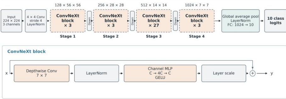
ConvNeXt-Base
