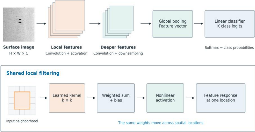
Figure 1. Shared local filtering and a generic CNN classification pipeline. The example input is a SteelDefectX10 test image; stacked feature maps are schematic and do not represent computed activations. A sliding kernel applies the same learned weights across locations before nonlinear transformation and subsequent aggregation.
