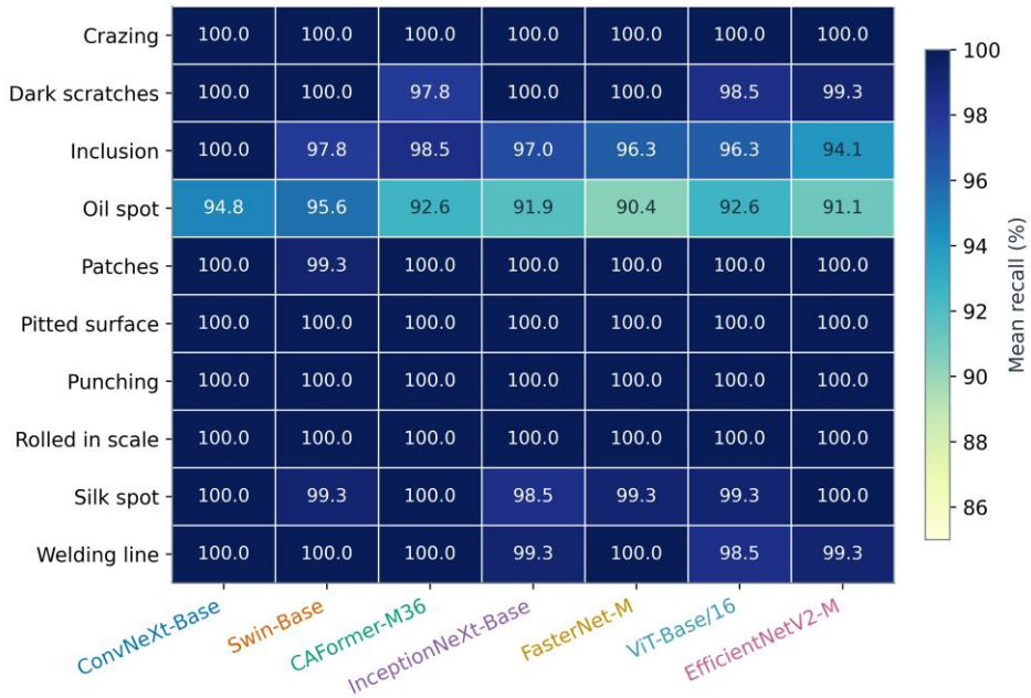
Figure 12. Class recall averaged across three seeds. Color and printed percentages show the recognition pattern over 45 unique images per class. The common scale spans 85% to 100%.
