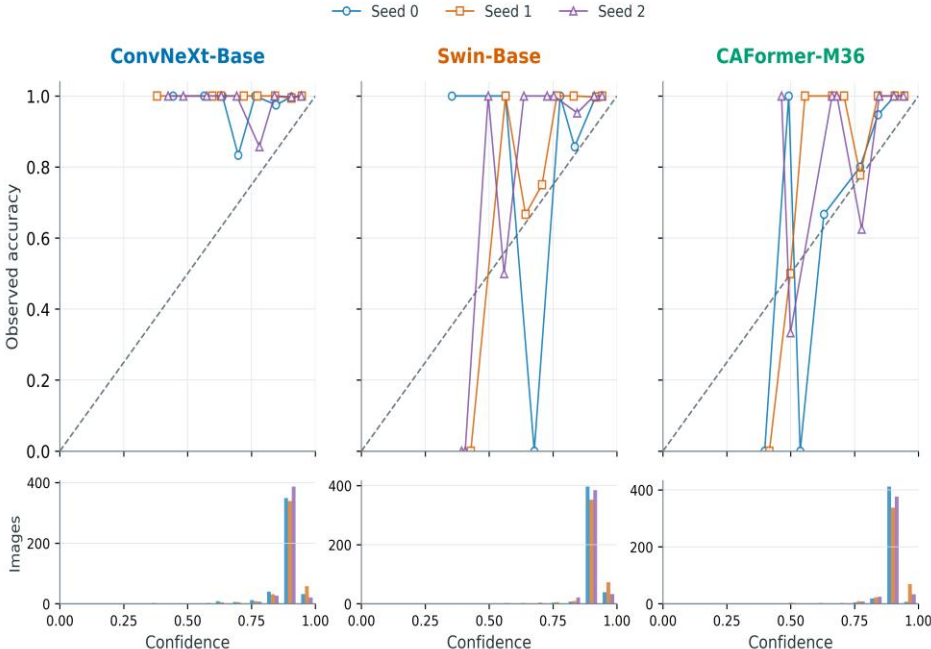
Figure 16. Reliability curves and confidence-bin populations for ConvNeXt, Swin, and CAFormer. Colors and open marker shapes identify seeds 0, 1, and 2. Curves use occupied bins among 15 equal-width confidence intervals; lower panels show image counts in each bin. The dashed line represents ideal calibration.
