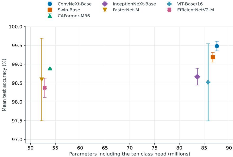
Figure 18. Model size and recognition accuracy. Model colors and marker shapes are consistent across comparison plots; vertical bars show the sample standard deviation across three seeds. Parameter counts include the ten-class classifier. Model size does not measure device latency or energy.
