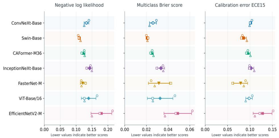
Figure 17. Probability quality for all seven pipelines. Filled model markers and horizontal bars show the mean and sample standard deviation over three seeds. Open circles, squares, and triangles show individual seeds 0, 1, and 2. Lower NLL, Brier, and ECE15 values are better; all quantities are dimensionless.
