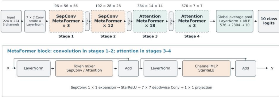
CAFormer-M36
