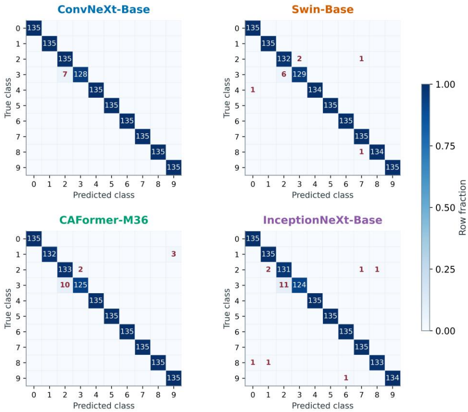
Figure 13a. Pooled confusion matrices for ConvNeXt, Swin, CAFormer, and InceptionNeXt. Rows are true classes and columns predicted classes. Blue intensity denotes the row fraction; printed values are counts. Each row comprises 135 predictions from repeated evaluation of 45 unique images.
