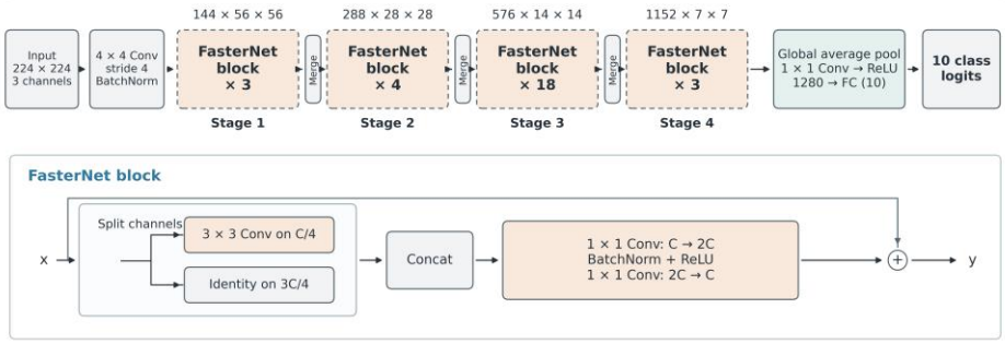
Figure 7. FasterNet-M for ten-class recognition. Four stages of partial-convolution blocks. One quarter of the channels receive standard spatial convolution, followed by pointwise channel mixing and a residual connection. Tensor labels in the hierarchy use C \times H \times W at a 224 \times 224 input. The diagrams omit training-time stochastic depth for clarity.
