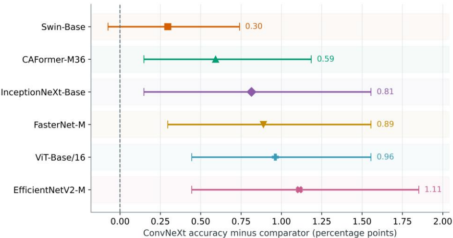
Figure 14. ConvNeXt minus each comparator in mean accuracy, with 95% paired class-stratified image-bootstrap percentile intervals. Intervals are conditional on the fitted seeds, exploratory, and unadjusted; the dashed line denotes zero. Printed values are mean differences in percentage points.
