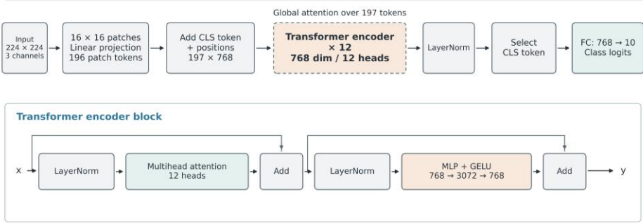
Figure 8. ViT-Base/16 for ten-class recognition. Patch projection and a twelve-block global-attention encoder. A class token aggregates the image sequence before the ten-class head; the inset shows both normalized residual sublayers. Tensor labels in the hierarchy use C \times H \times W at a 224 \times 224 input. The diagrams omit training-time stochastic depth for clarity.
