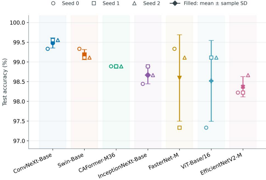
Figure 11. Test accuracy across three training seeds. Open circles, squares, and triangles identify seeds 0, 1, and 2. Filled model markers and error bars show the mean and sample standard deviation; colors distinguish pipelines. All runs use the same 450 test images.
