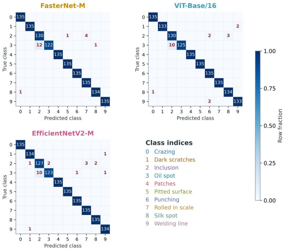
Figure 13b. Pooled confusion matrices for FasterNet, ViT, and EfficientNetV2, with the common class-index legend. Nonzero errors are printed in red. Counts pool three seeds on the same 45 unique images per class, rather than additional independent test images.
