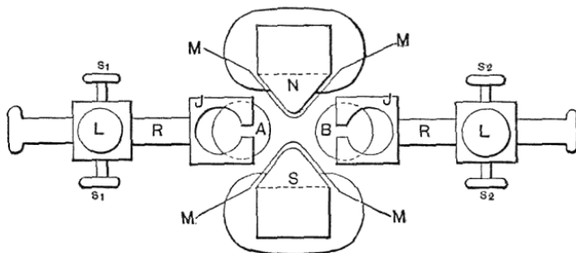
FIG. 4.—ARRANGEMENT OF IMPROVED DISCHARGER AND MAGNET.
