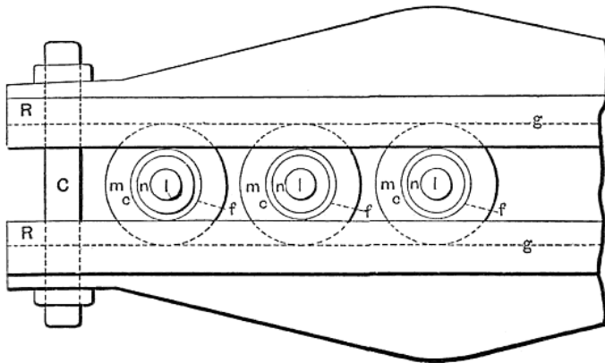
FIG. 7.—DISCHARGER WITH MULTIPLE GAPS.
