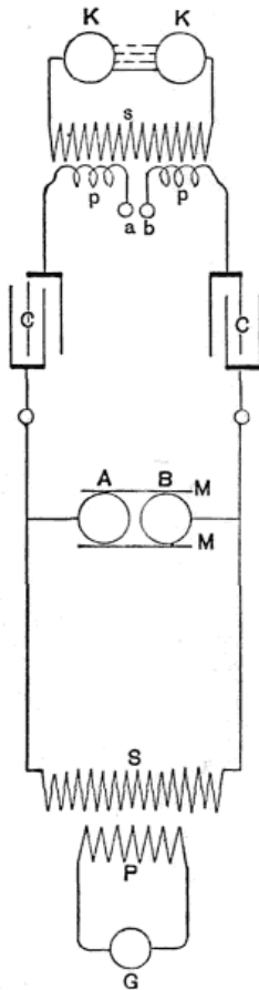
FIG. 2.—IMITATING THE SPARK OF A HOLTZ MACHINE.
