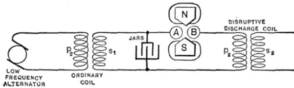
FIG. 5.—ARRANGEMENT WITH LOW-FREQUENCY ALTERNATOR AND IMPROVED DISCHARGER.
