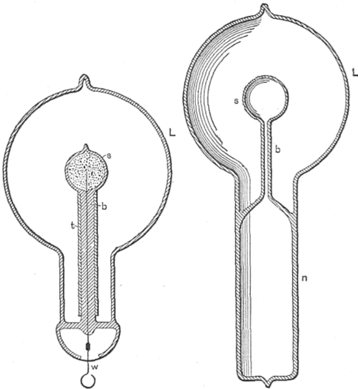
FIG. 12. FIG. 13. BULBS FOR PRODUCING ROTATING BRUSH.
