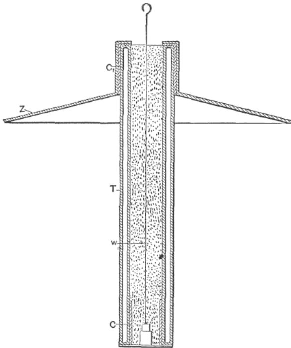
FIG. 27.—PHOSPHORESCENT TUBE WITH INTENSIFYING REFLECTOR.
