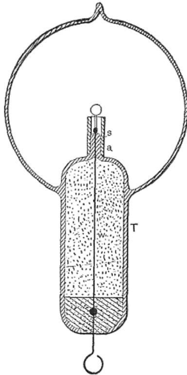
FIG. 21.—IMPROVED BULB WITH NON-CONDUCTING BUTTON.
