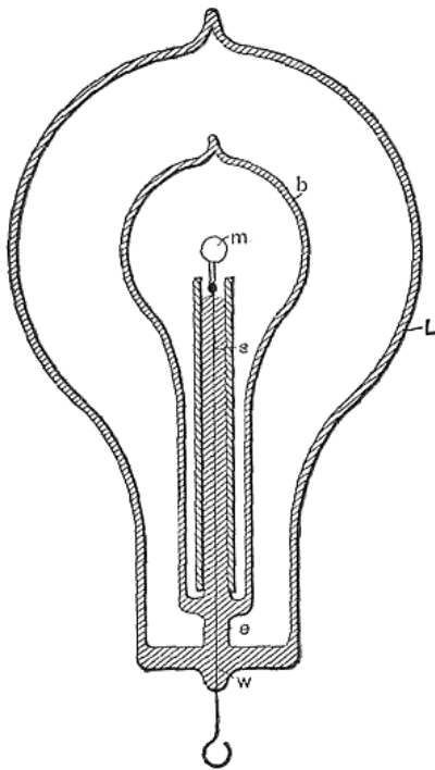
FIG. 29.—LAMP WITH INDEPENDENT AUXILIARY BULB.
